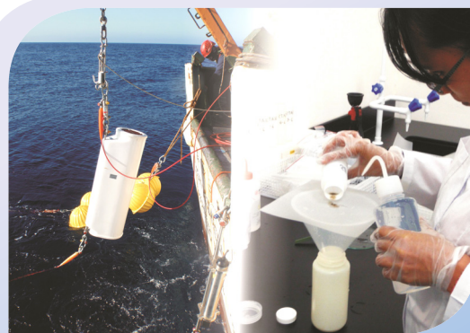
An anchored collector is prepared on the deck of SEATS
